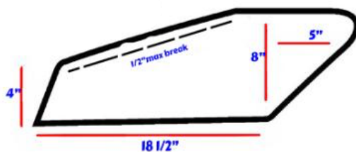
MAXIMUM of 3 spoiler Blades
